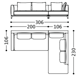
01BOWC2 (1BOW210SX + 1BOW260DX) 02BOWC2 (2BOW210SX + 2BOW260DX)
