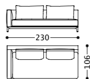
1BOW220SX 2BOW220SX
